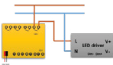
1. Non-dimmable Driver
